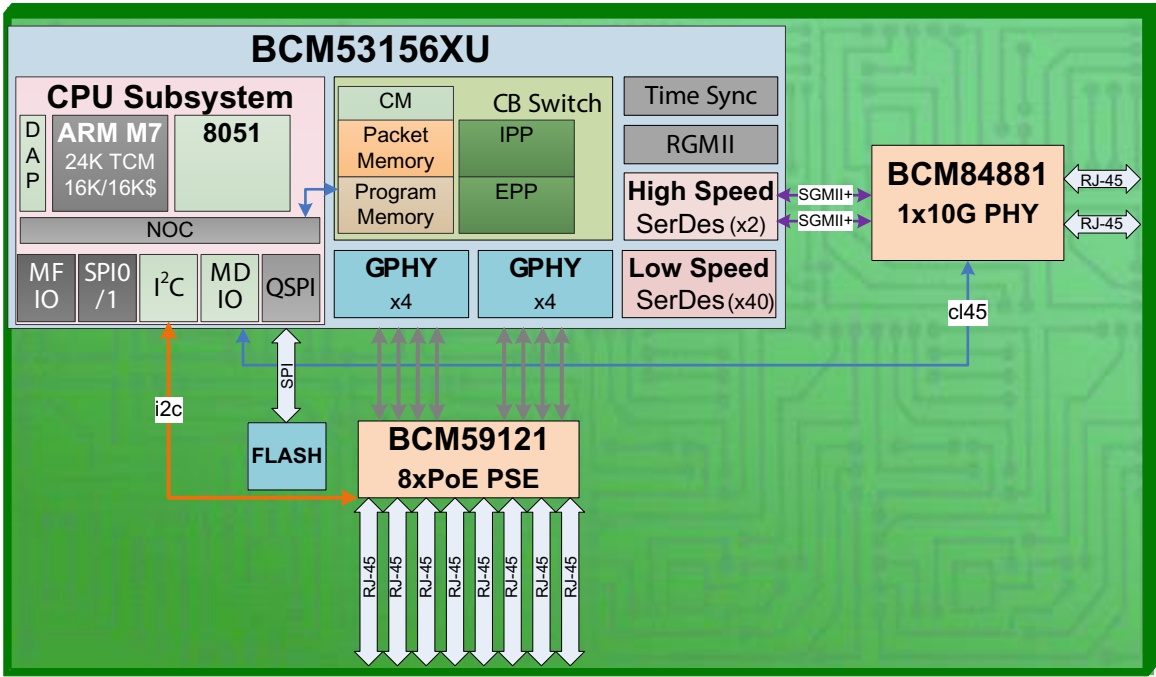
Figure 6: High-Speed Unmanaged
