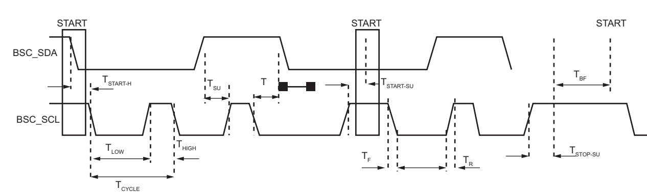
Figure 34: BSC Interface
