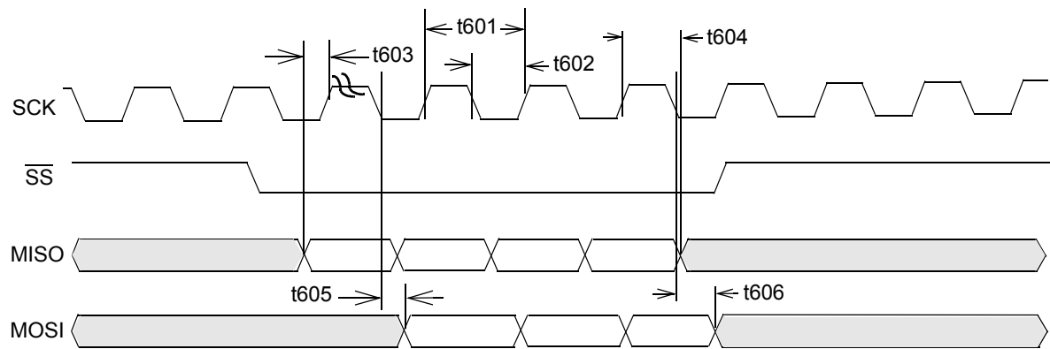
Figure 31: SPI-1 Timing, \overline{SS} Asserted During SCK High
