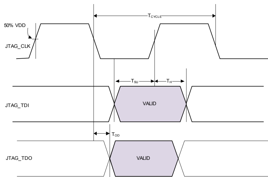
Figure 33: JTAG Interface
