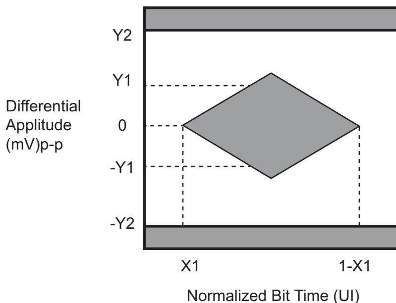
Figure 20: XFI Far-End Eye Mask
