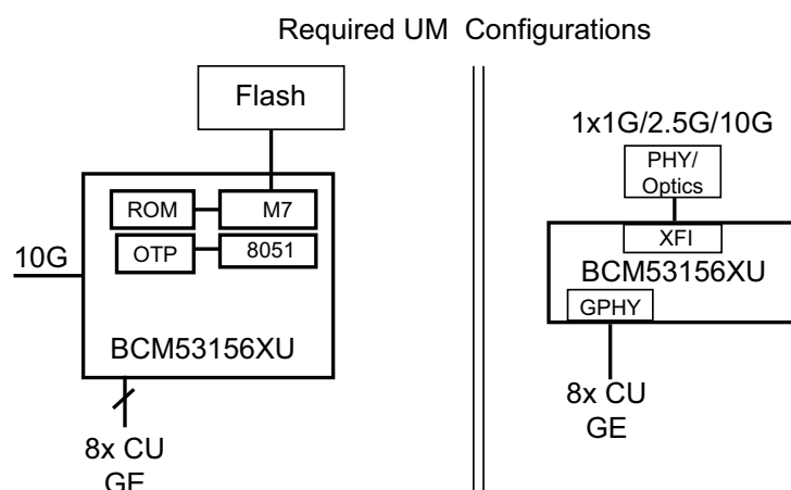
Figure 4: Unmanaged Applications
