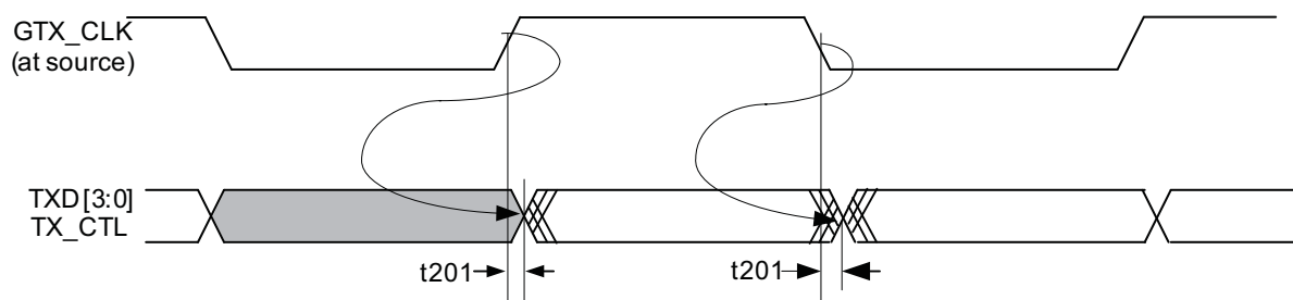
Figure 22: RGMII Output Timing (Normal Mode)
