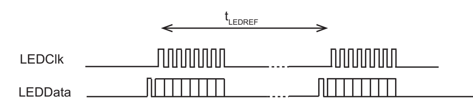
Figure 36: LEDCk/LEDData Refresh Interval
